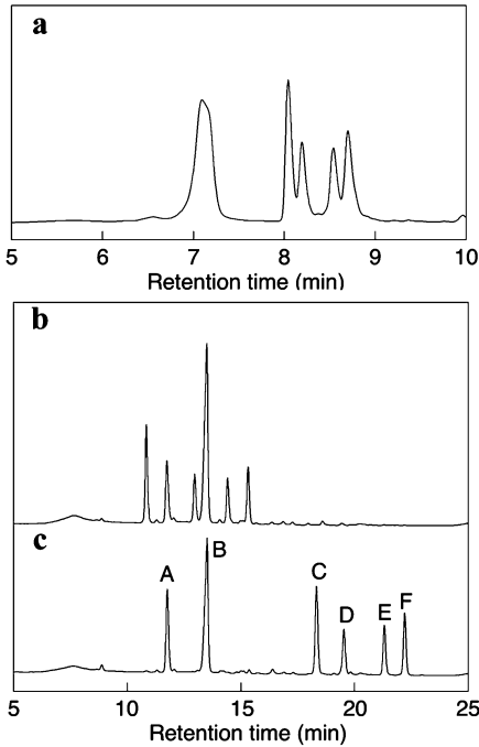
FIGURE 5 HPLC analyses of the dimer fraction produced by clay-catalyzed oligomerization of racemic ImpA in imidazole buffer. (a) Anion exchange, and reversed phase HPLC chromatograms (b) before and (c) after alkaline phosphatase treatment of the dimer fraction.
