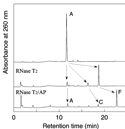
FIGURE 6 Reversed phase HPLC analyses of RNase T 2 followed by alkaline phosphatase (AP) treatment of dimer A.
