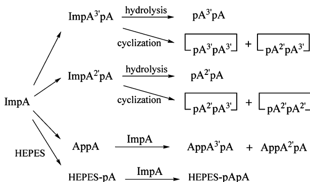
FIGURE 3 Possible dimer products formed by the condensation reaction of D-ImpA catalyzed by Na + -montmorillonite. In the reaction of racemic ImpA, additional enantio- and diastereo-isomers are formed.
