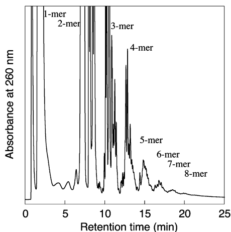
FIGURE 2 An anion exchange HPLC chromatogram of montmorillonite-catalyzed oligomerization products of racemic ImpA.
