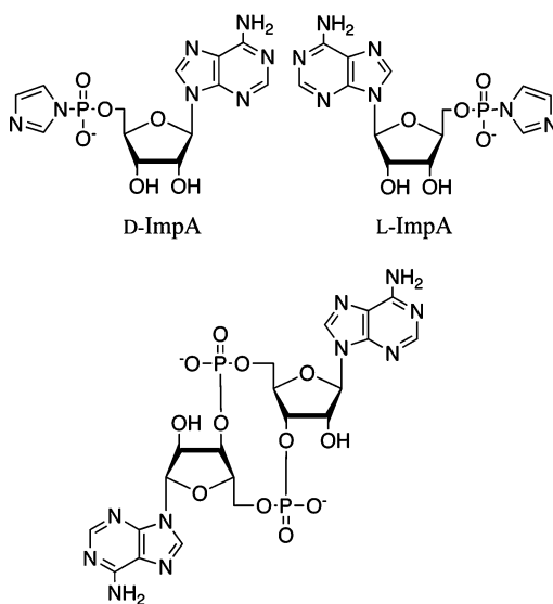
FIGURE 1 Structures of D-, L-ImpA (upper) and D-homochiral cyclic pA 3' pA 3' (bottom).
