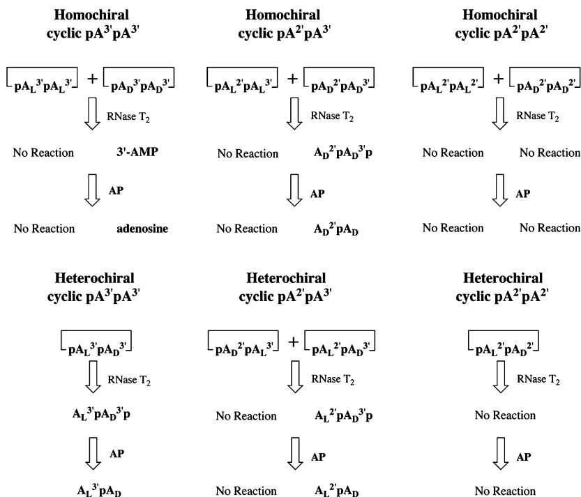
FIGURE 7 Regio-, enantio-, and diastereo-isomers of cyclic adenylyl-adenosine, and their expected degradation products with RNase T 2 and alkaline phosphatase (AP) treatments. Since heterochiral cyclic pA L 3' pA D 3' and cyclic pA L 2' pA D 2' are mesomeric, their enantiomers do not exist.
