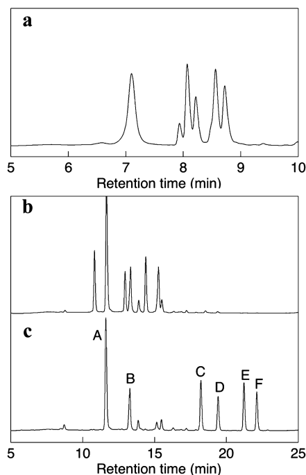
FIGURE 4 HPLC analyses of the dimer fraction produced by clay-catalyzed oligomerization of racemic ImpA in HEPES buffer. (a) Anion exchange, and reversed phase HPLC chromatograms (b) before and (c) after alkaline phosphatase treatment of the dimer fraction.
