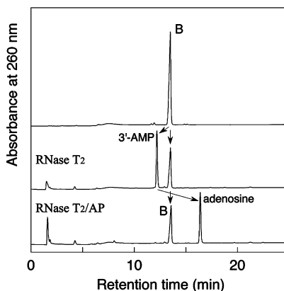
FIGURE 8 Reversed phase HPLC analyses of RNase T 2 followed by alkaline phosphatase (AP) treatment of dimer B.
